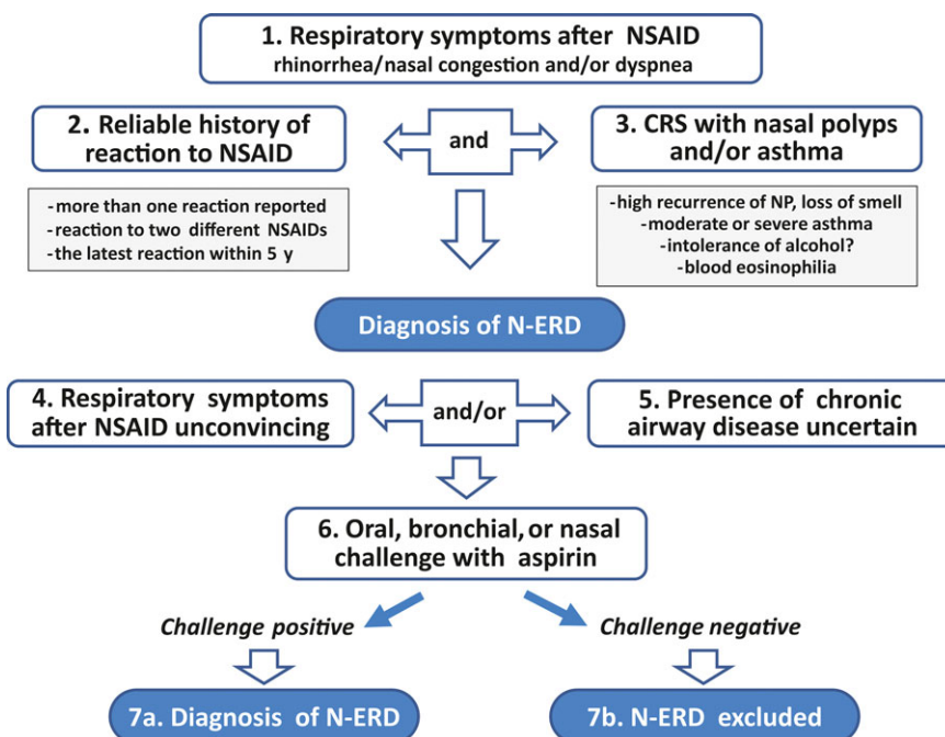
FIGURE 2 Algorithm for diagnosis of N-ERD (description in the text)
