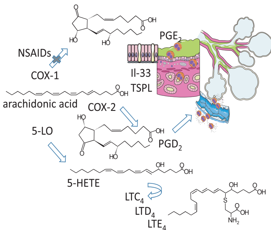
FIGURE 1 Pathomechanisms of N-ERD. In response to non-specific, unknown factors, respiratory epithelium overproduces innate immunity type 2 mediators (e.g. interleukin-33 (IL-33), thymic stromal lymphopoietin-TSPL) attracting eosinophils. Inhibition of cyclooxygenase-1 (COX-1) by NSAIDs decreases biosynthesis of prostaglandin E 2 (PGE 2 ) from arachidonic acid. Deficiency of this anti-inflammatory mediator is not compensated by the inducible isoenzyme COX-2, which produces chemoattractant prostaglandin D 2 (PGD 2 ). Excess of arachidonate substrate is metabolized by 5-lipoxygenase (5-LO) to leukotrienes (LTC 4 , LTD 4 , and LTE 4 ), potent pro-inflammatory mediators. Eosinophils and possibly granulocyte-platelet aggregates accumulate at the bronchi perpetuating these specific alterations in the lipid mediators of asthma
